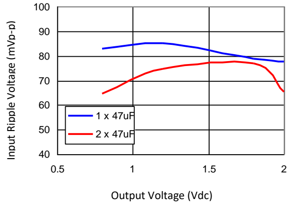
Figure 28. Input ripple voltage for various output voltages with 1 \times 47\mu F or 2 \times 47\mu F ceramic capacitors at the input (30A load). Input voltage is 3.3V.
