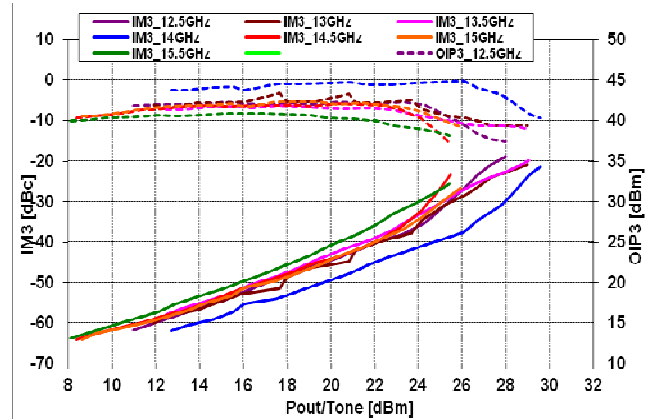
@Vds=5V, Ids=1400mA
