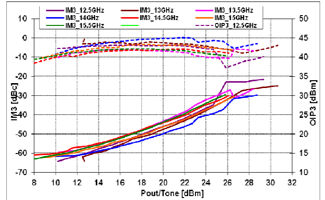
@Vds=6V, Ids=1400mA
