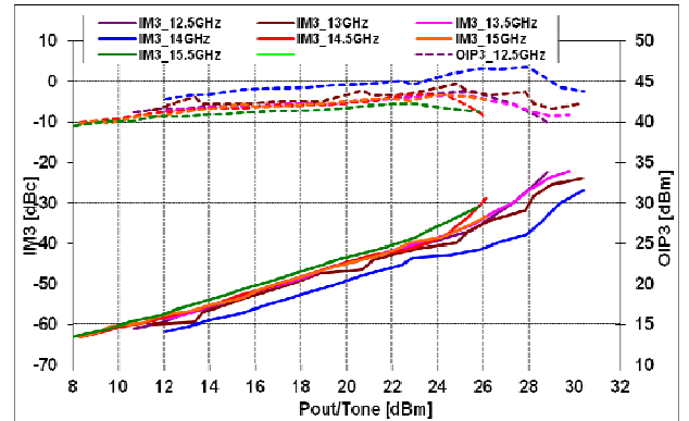
@Vds=6V, Ids=2000mA
