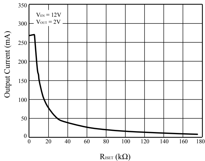
Figure 11 Output Current vs. R_{SET}
