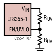
Figure 7. LT8355-1 Resistor Network for Accurate UVLO.
