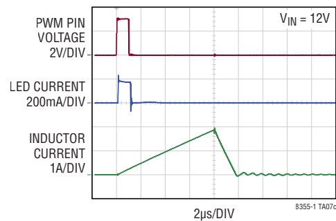
10000:1 External PWM Dimming at 100Hz
