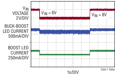
Cold Crank LED Regulation
