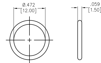
O-RING
