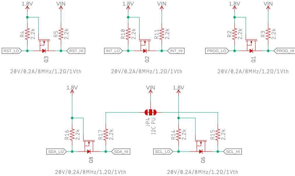
Logic-Level Conversion
