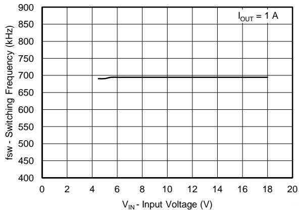
Figure 20. V OUT 1 = 3.3V Switching Frequency vs Input Voltage
