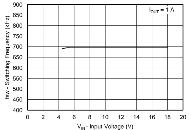
Figure 21. V OUT 2 = 1.2V Switching Frequency vs Input Voltage
