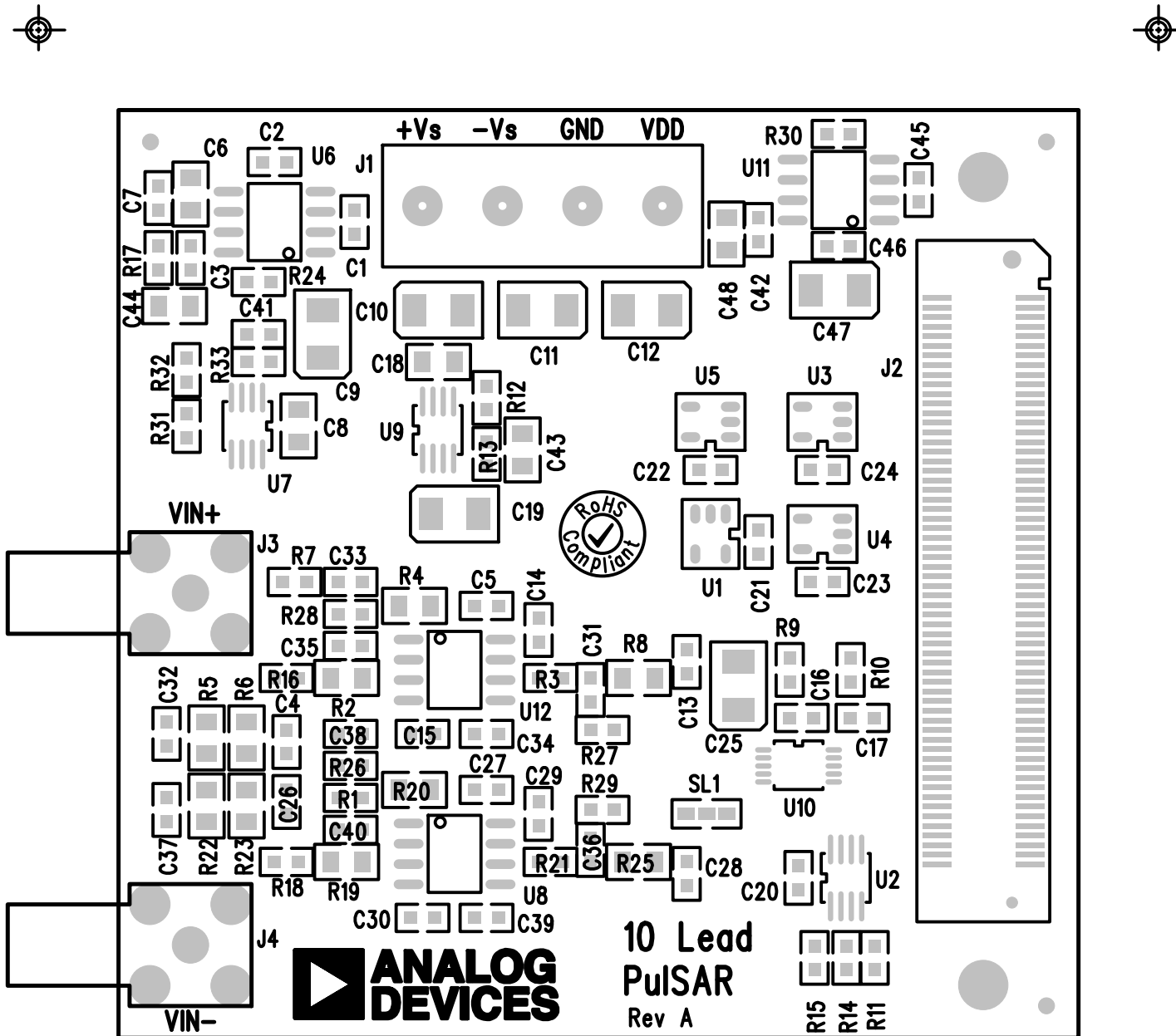
10 Lead PuLSAR Rev. A - Top Side View. Silkscreen Top
