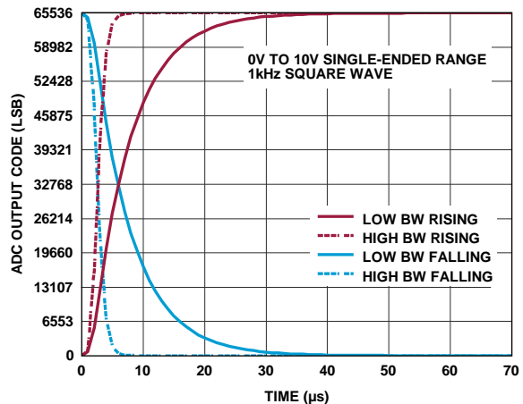
Figure 65. Step Response, 0 V to 10 V Single-Ended Range
