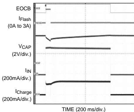
Figure 26. 5.3-V Mode Super Capacitor Charge
