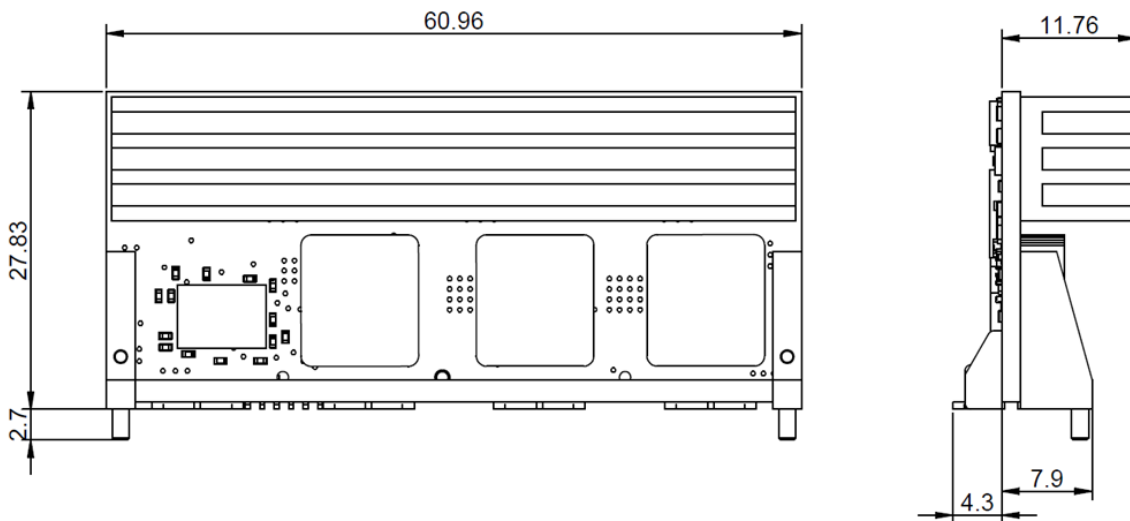
Figure 51. Mechanical Drawing (Unit: mm [inch])
