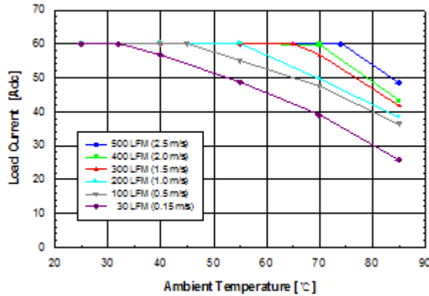
Figure 5. Thermal Derating Curves. Vin=12V, Vout=2.5V
