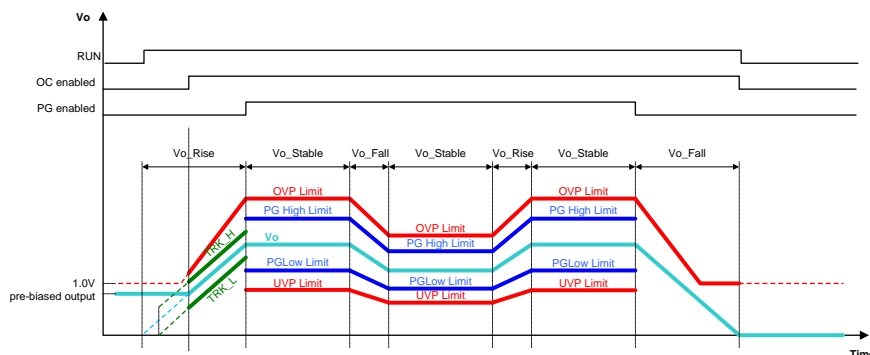
Figure 25. Protections Enable Conditions
