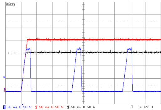
Figure 32. Turn-On into UVP on V3. The UV Fault is programmed to be Non-Latching. Ch1 - Vo1, Ch2 - Vo2 (Group A), Ch3 - Vo3 (Group B). Vo4 not shown.
