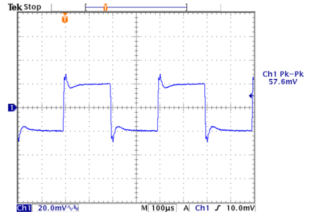
Figure 10. Transient Response with Optimal Voltage Positioning
