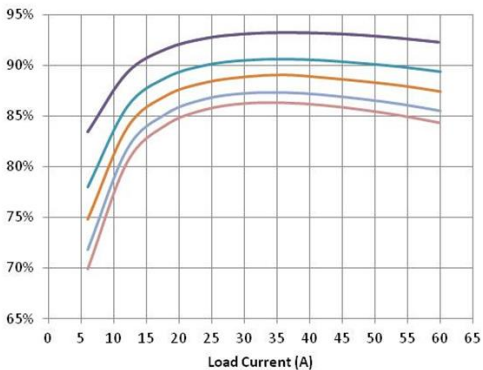
Figure 3. Efficiency vs Load at Vin = 12V
