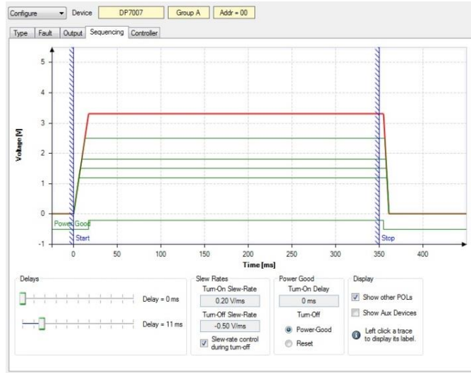
Figure 11. Sequencing/Tracking Window
