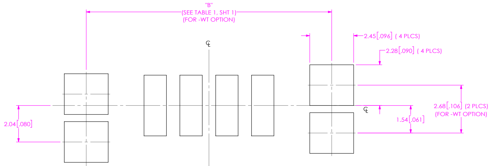
FIG 2 UMPT-04-XX.X-X-VT-SM-X-WT-X STENCIL SHOWN (DIFFERENT AS SHOWN, OTHERWISE SAME AS FIG 1)
