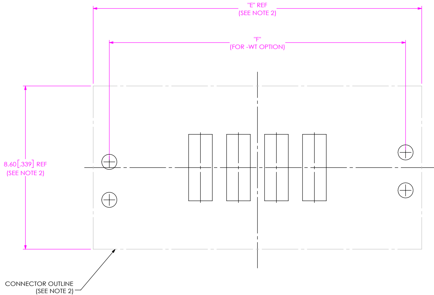
FIG 5 UMPT-04-XX.X-X-VT-SM-X-WT-M-X FOOTPRINT SHOWN (DIFFERENT AS SHOWN, OTHERWISE SAME AS FIG 1)
