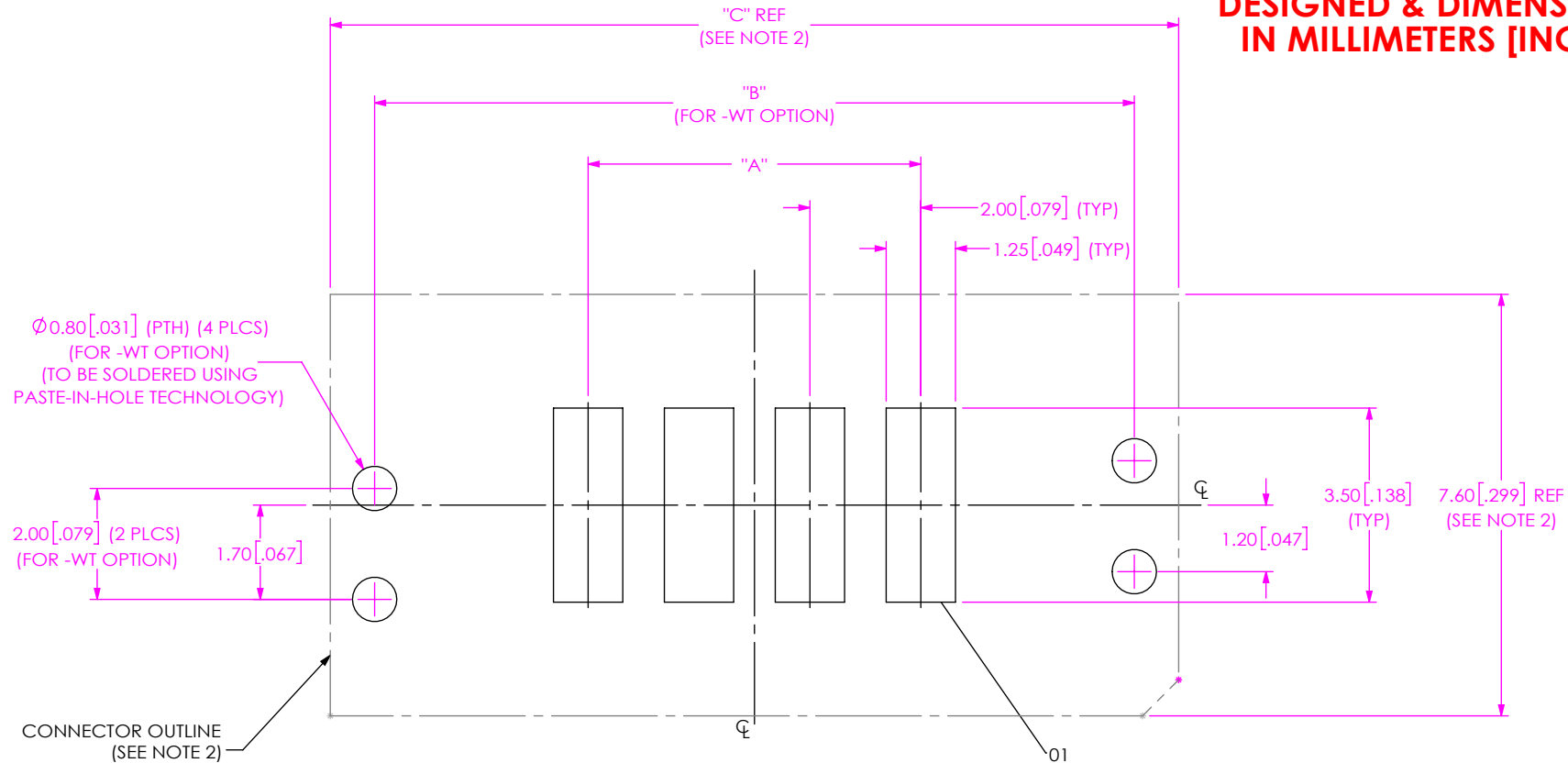
FIG 1 UMPT-04-XX.X-X-VT-SM-X-WT-X FOOTPRINT SHOWN
