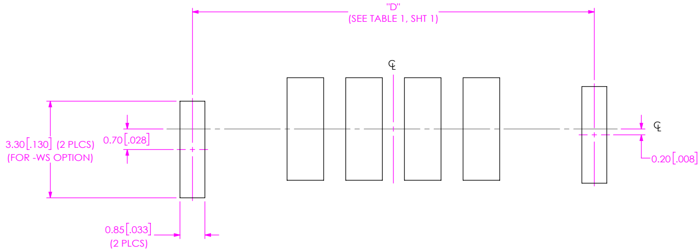
FIG 4 UMPT-04-XX.X-X-VT-SM-X-WS-X STENCIL SHOWN (DIFFERENT AS SHOWN, OTHERWISE SAME AS FIG 1 & 3)
