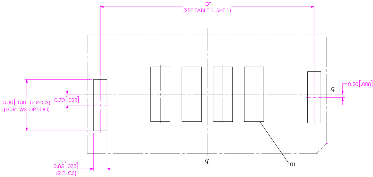
FIG 3 UMPT-04-XX.X-X-VT-SM-X-WS-X FOOTPRINT SHOWN (DIFFERENT AS SHOWN, OTHERWISE SAME AS FIG 1)
