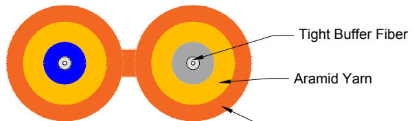
Cable Structure
