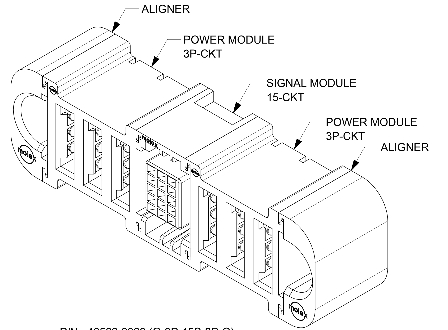
P/N : 46562-9323 (G-3P-15S-3P-G)
