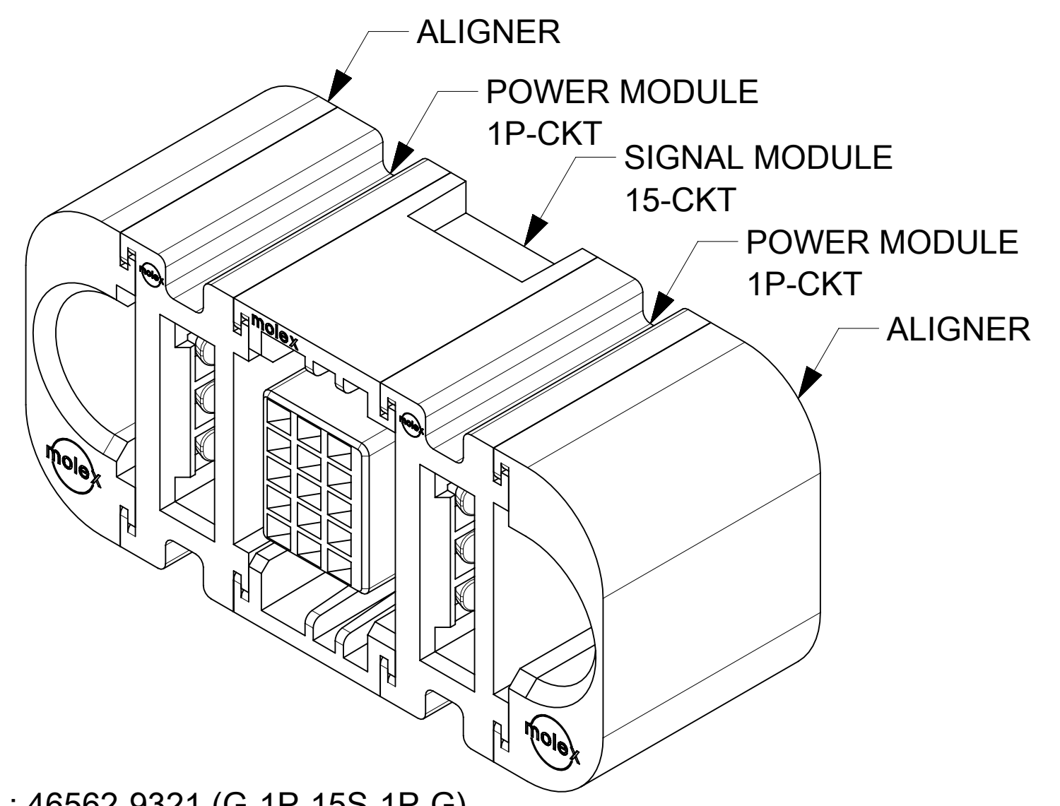
P/N : 46562-9321 (G-1P-15S-1P-G)
