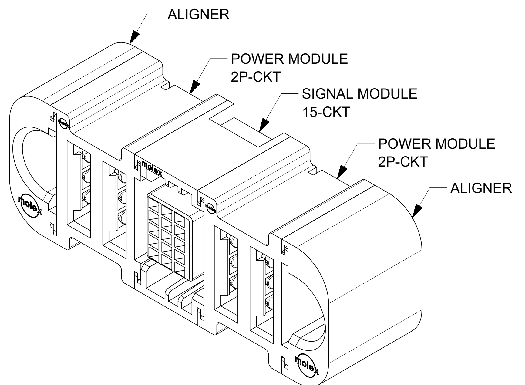
P/N : 46562-9322 (G-2P-15S-2P-G)
