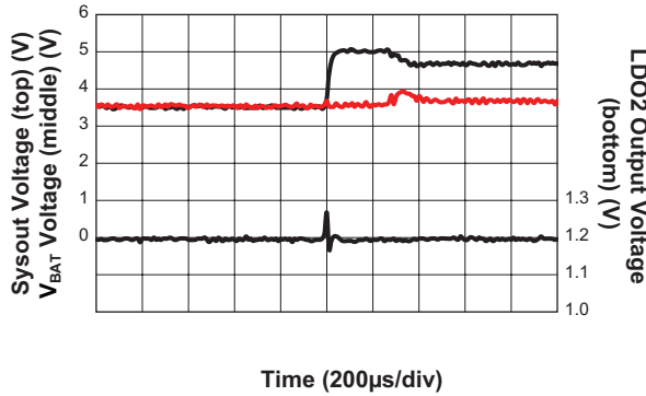
System Line Transient Response ( V_{IN} = 3.5V to 5V ; V_{BAT} = 3.6V ; V_{LDO2} = 1.2V ; I_{LDO2} = 80mA ; rising)
