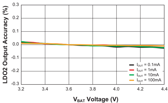
Line Regulation ( V_{LDO2} = 1.2V )
