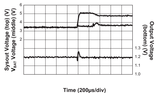
System Line Transient Response ( V_{IN} = 3.5V to 5V ; V_{BAT} = 3.6V ; V_{OUTB2} = 1.2V ; I_{OUTB2} = 800mA ; rising)
