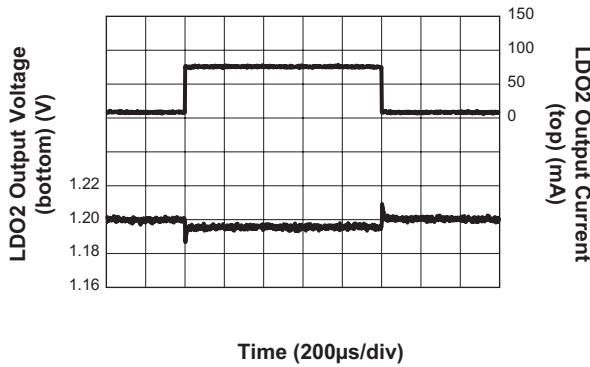
Load Transient Response ( I_{LDO2} = 8mA to 80mA ; V_{BAT} = 3.6V ; V_{LDO2} = 1.2V ; C_{LDO2} = 4.7µF )
