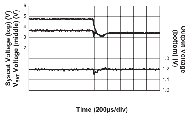
System Line Transient Response ( V_{IN} = 3.5V to 5V ; V_{BAT} = 3.6V ; V_{OUTB2} = 1.2V ; I_{OUTB2} = 800mA ; falling)
