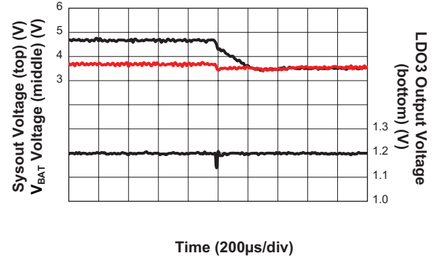
System Line Transient Response ( V_{IN} = 3.5V to 5V ; V_{BAT} = 3.6V ; V_{LDO3} = 1.2V ; I_{LDO3} = 80mA ; falling)
