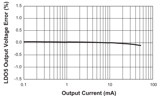
Load Regulation ( V_{BAT} = 3.6V ; V_{LDO5} = 3.3V )
