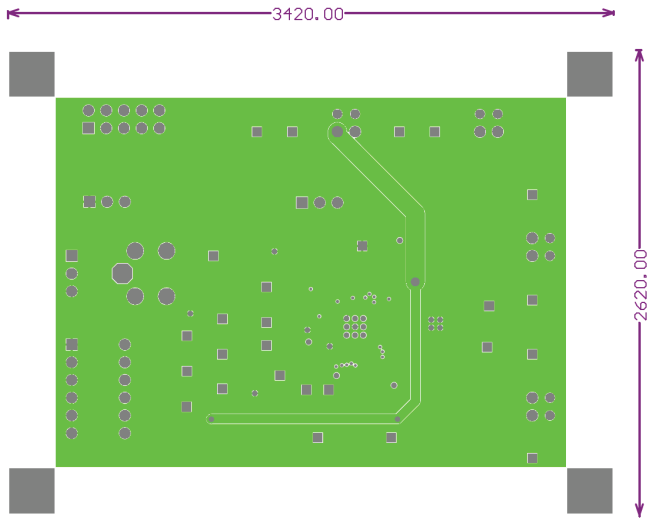
Figure 14: AAT3608 Evaluation Board
