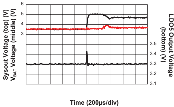
System Line Transient Response ( V_{IN} = 3.5V to 5V ; V_{BAT} = 3.6V ; V_{LDO5} = 3.3V ; I_{LDO5} = 50mA ; rising)
