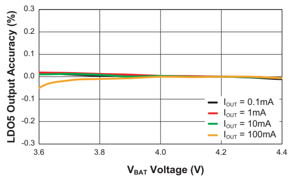
Line Regulation ( V_{LDO5} = 3.3V )
