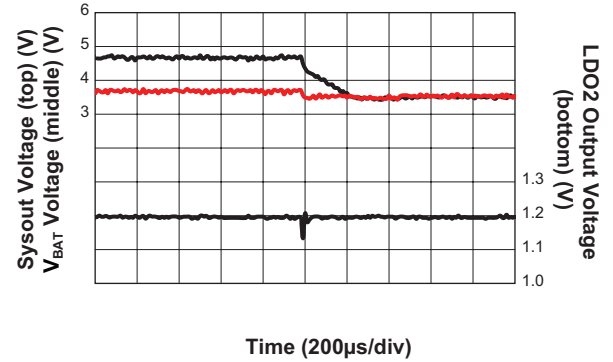
System Line Transient Response ( V_{IN} = 3.5V to 5V ; V_{BAT} = 3.6V ; V_{LDO2} = 1.2V ; I_{LDO2} = 80mA ; falling)
