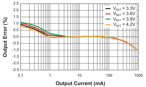
DC Regulation vs. Load ( V_{B2} = 1.2V ; L_2 = 2.2\mu H )
