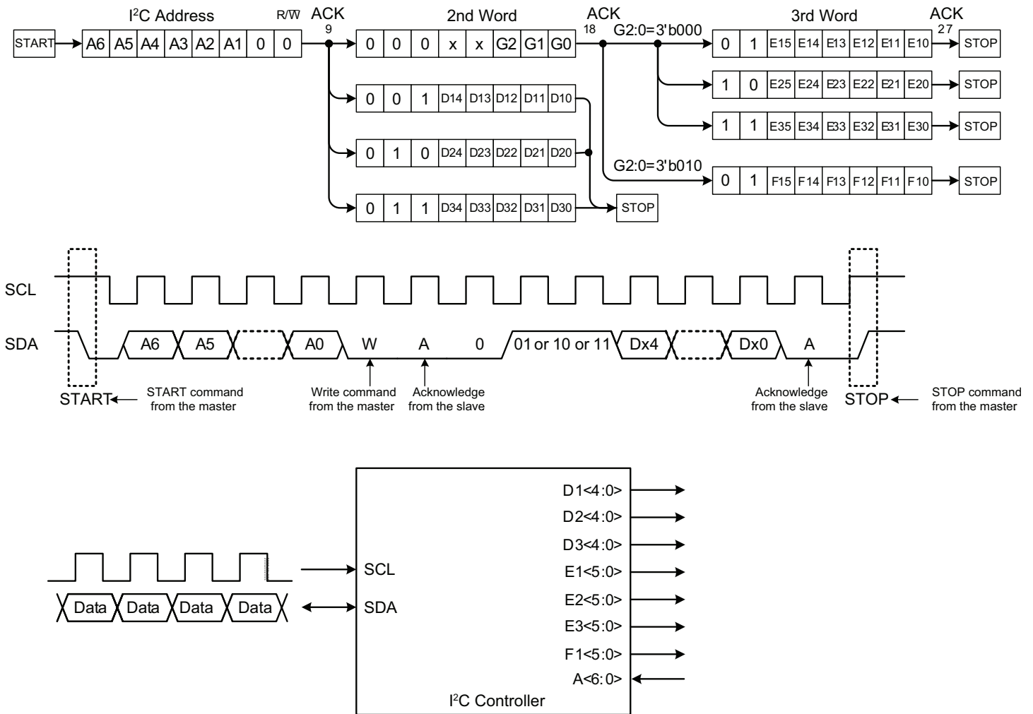
Figure 9: I2C Protocol.
