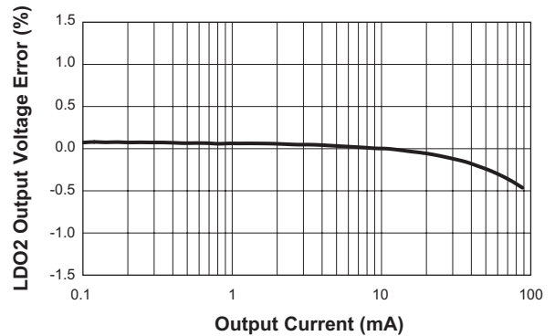
Load Regulation ( V_{BAT} = 3.6V ; V_{LDO2} = 1.2V )
