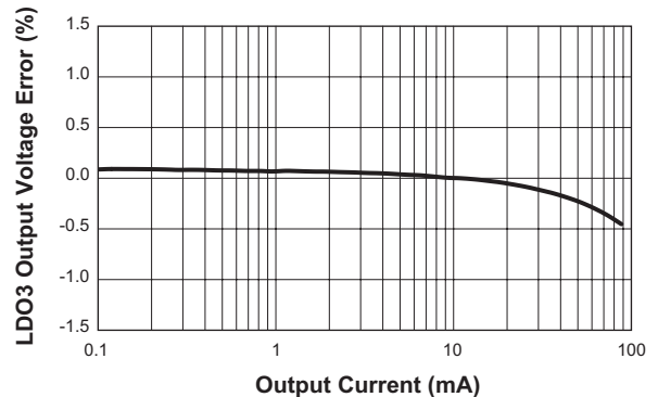
Load Regulation ( V_{BAT} = 3.6V ; V_{LDO3} = 1.2V )
