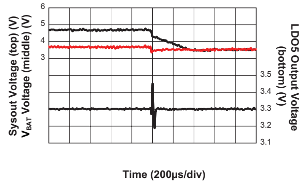
System Line Transient Response ( V_{IN} = 3.5V to 5V ; V_{BAT} = 3.6V ; V_{LDO5} = 3.3V ; I_{LDO5} = 50mA ; falling)
