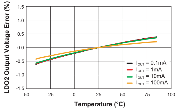
Output Voltage Error vs. Temperature ( V_{BAT} = 3.6V ; V_{LDO2} = 1.2V )
