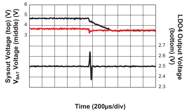
System Line Transient Response ( V_{IN} = 3.5V to 5V ; V_{BAT} = 3.6V ; V_{LDO4} = 2.5V ; I_{LDO4} = 50mA ; falling)
