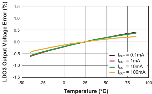
Output Voltage Error vs. Temperature ( V_{BAT} = 3.6V ; V_{LDO3} = 1.2V )
