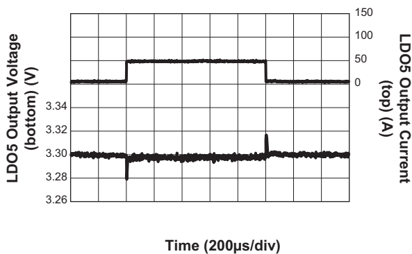
Load Transient Response ( I_{LDO5} = 5mA to 50mA ; V_{BAT} = 3.9V ; C_{LDO5} = 4.7µF )
