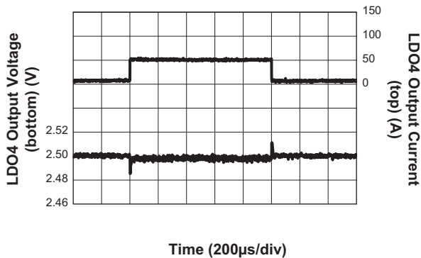
Load Transient Response ( I_{LDO4} = 5mA to 50mA ; V_{BAT} = 3.6V ; V_{LDO4} = 2.5V ; C_{LDO4} = 4.7µF )
