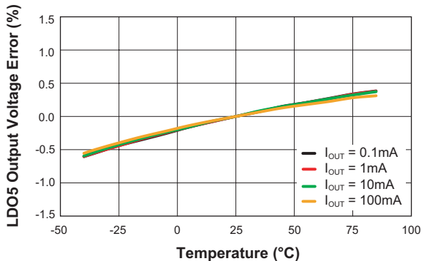
Output Voltage Error vs. Temperature ( V_{BAT} = 3.6V ; V_{LDO4} = 3.3V )
