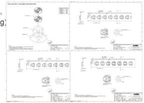
Add carrier tape drawing in sheet 2-4
