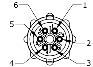
WIRING VIEW W18980-6SG-P-5XX
