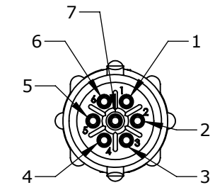
WIRING VIEW W18980-7SG-P-5XX
