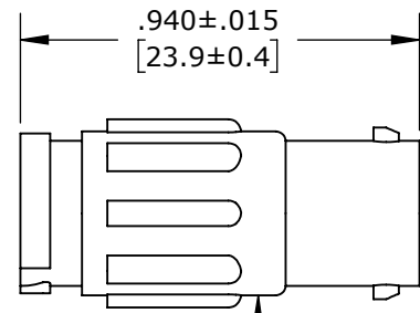
CABLE TO CABLE HOUSING MAT'L: HOUSING -THERMOPLASTIC, BLACK
