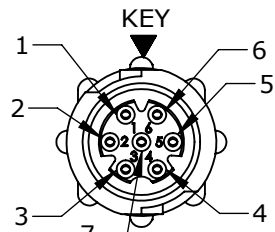
FACE VIEW W18980-7SG-P-5XX 7 POSITION
