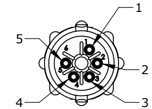
WIRING VIEW W18980-5SG-P-5XX
