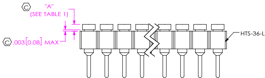
FIG. 2 HSS-1XX-XX-2-N SHOWN (SAME AS FIG 1, DIFFERENT AS SHOWN)
