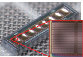
Thermopile
