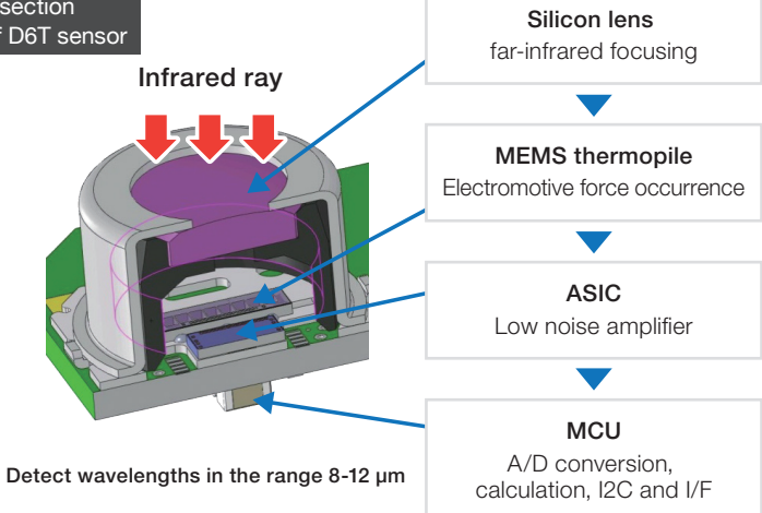
MEMS thermopile
