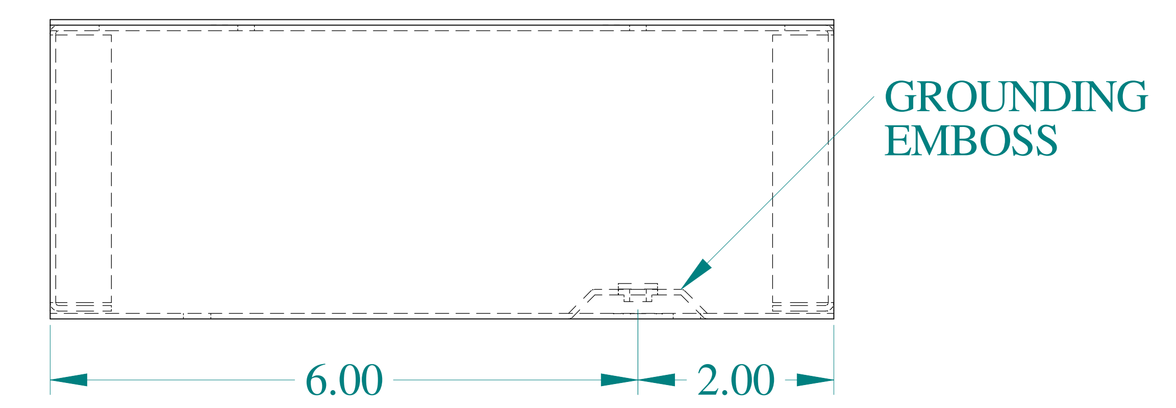
SIDE VIEW
