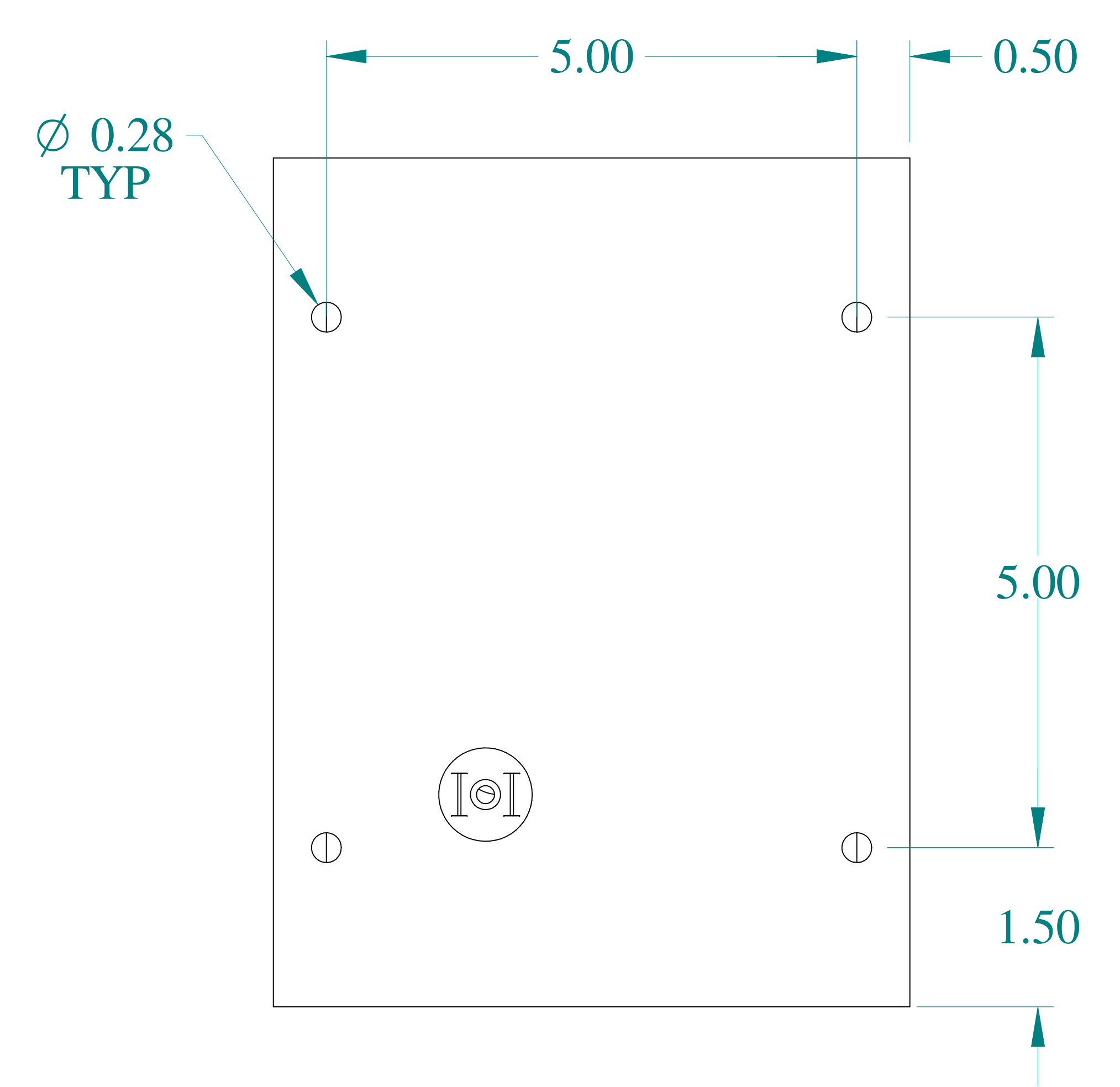
BOTTOM VIEW
