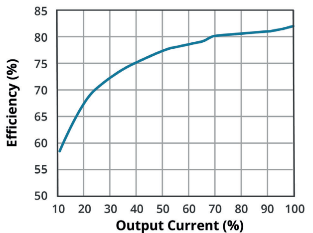
EFFICIENCY VS OUTPUT LOAD AE15-UW-S24
