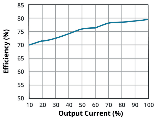
EFFICIENCY VS OUTPUT LOAD AE15-UW-S15
