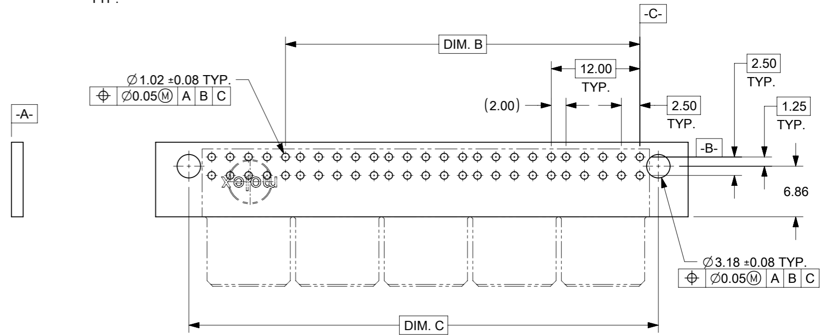
PCB LAYOUT: COMPONENT SIDE (PEG HOLES OPTIONAL)
