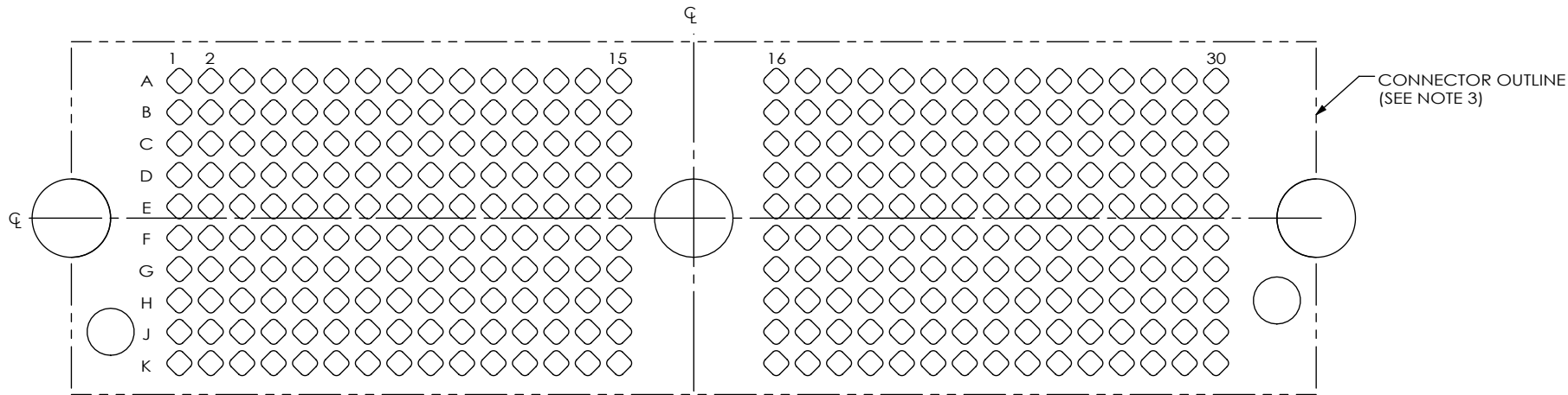
FIG 4 ZA8-30-2-1.00-X-10 TOP MATING PCB SHOWN (DUAL COMPRESSION) (DIFFERENT AS SHOWN, OTHERWISE SAME AS FIG 2 & 3) (ALSO APPLIES TO ZA8-40)
