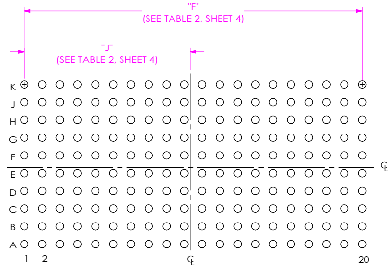
FIG 10 ZA8-20-1-1.00-X-10-X BOTTOM STENCIL SHOWN (SINGLE COMPRESSION STENCIL)
