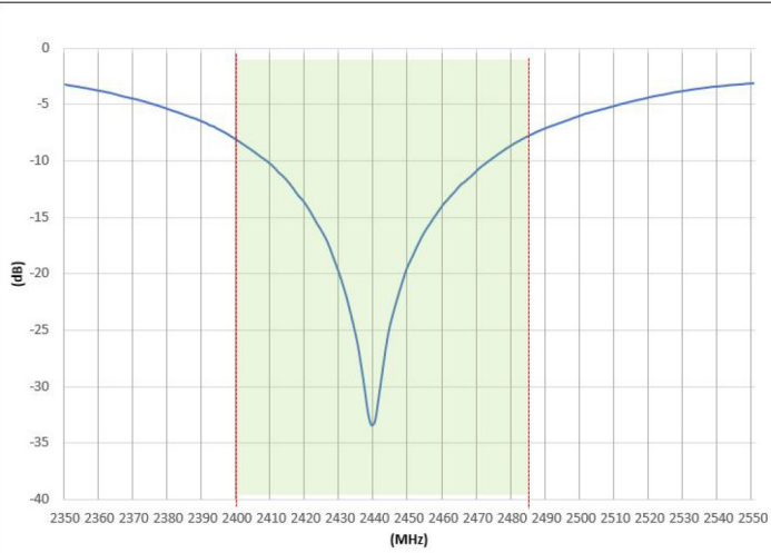
Return Loss
