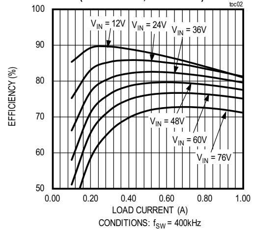
EFFICIENCY vs. LOAD CURRENT (3.3V OUTPUT, PWM MODE)
