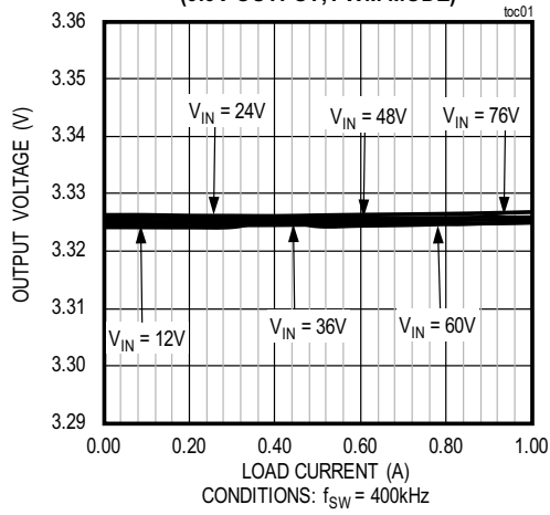
LOAD AND LINE REGULATION (3.3V OUTPUT, PWM MODE)
