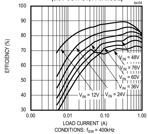
EFFICIENCY vs. LOAD CURRENT (3.3V OUTPUT, PFM MODE)
