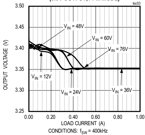
LOAD AND LINE REGULATION (3.3V OUTPUT, PFM MODE)
