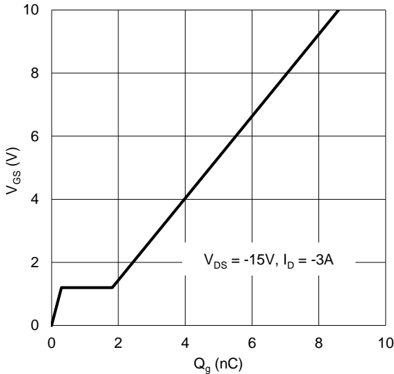
Figure 23. Gate Charge
