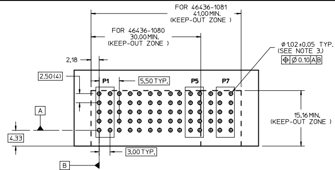
RECOMMENDED PCB LAYOUT AND KEEP-OUT ZONE
