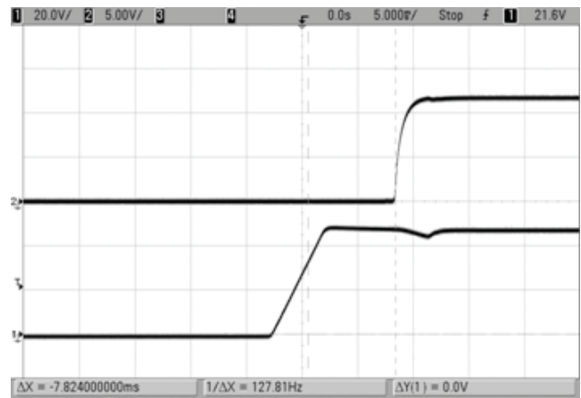
Start up Delay (Vin=48V, Iout=20A, Load=470uF, Ta=+25°C) Ch1=Vin, Ch2=Vout
