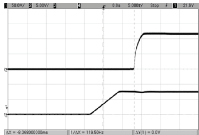
Start up Delay (Vin=48V, Iout=20A, Load=4700uF, Ta=+25°C) Ch1=Vin, Ch2=Vout
