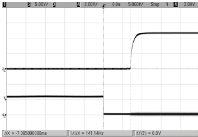
On/Off Enable start up (Vin=48V, Iout=20A, Load=4700uF, Ta=+25°C) Ch2=Vout, Ch4=Enable
