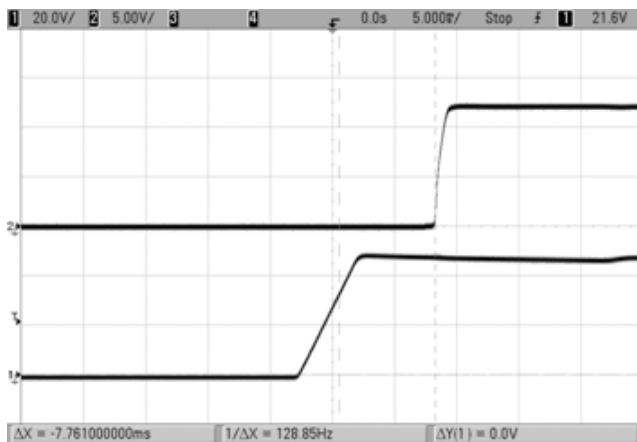
Start up Delay (Vin=48V, Iout=0A, Load=470uF, Ta=+25°C) Ch1=Vin, Ch2=Vout
