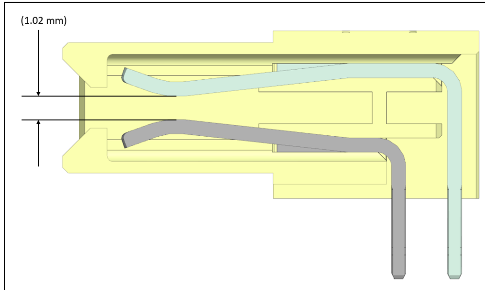
Hybrid Right-Angle Receptacle
