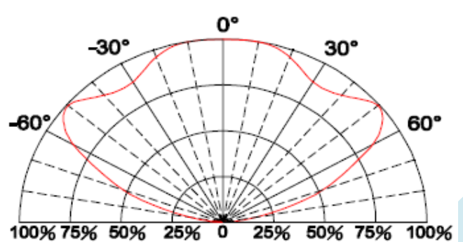
Fig.6 Directive Radiation
