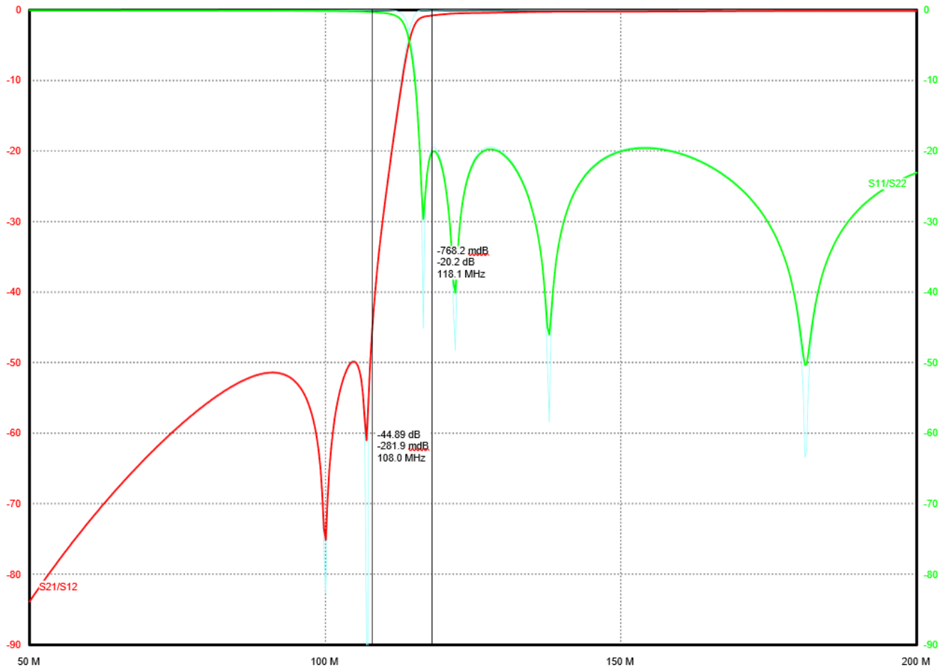
Lumped Filter S Parameters
