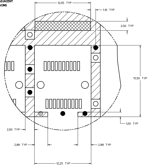
DETAIL 1 SCALE 8:1
