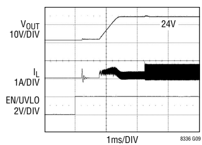
Switching Waveforms, Soft-Start
