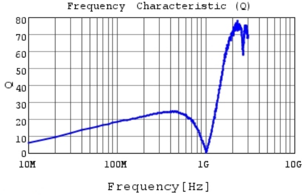
LQG15WHR15G02 Q
