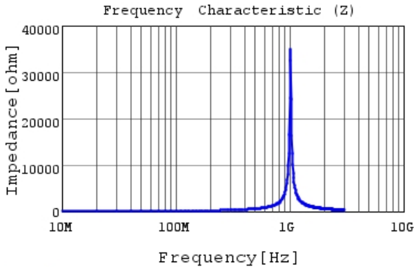
LQG15WHR15G02 |Z|
