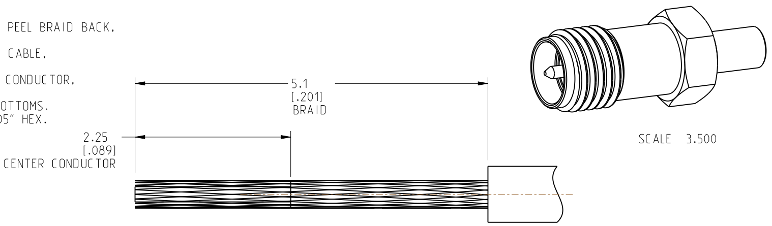
RECOMMENDED CABLE STRIPPING DIMENSIONS
