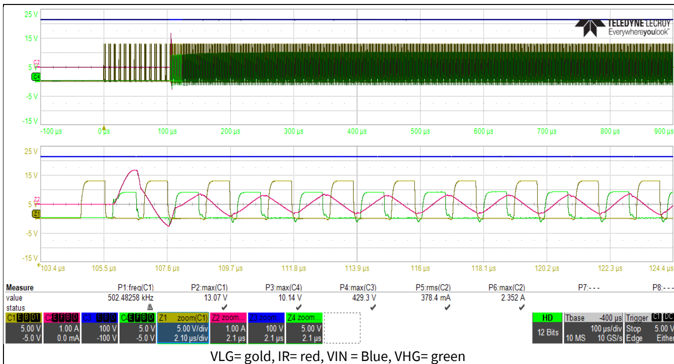
Figure 21 Burst mode zoomed at 425 V, no load: peak current of 2.35 A
