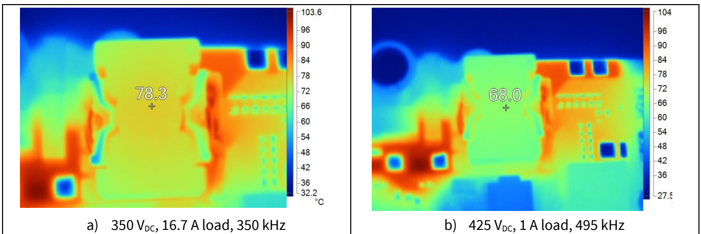
Figure 24 Temperature measurements of transformer – top side
