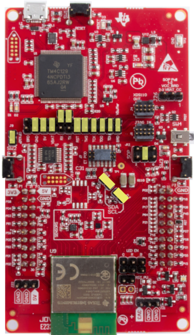
Figure 10. MOD LaunchPad Jumper Settings
