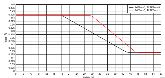
Figure 116. 1x Mode (2xFBn = 0) Foldback Curves, I PORT vs V DRAIN
