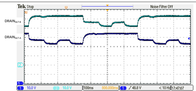
Figure 134. 4-Pair High Resistance ( 36\text{k}\Omega ) Detection Signature
