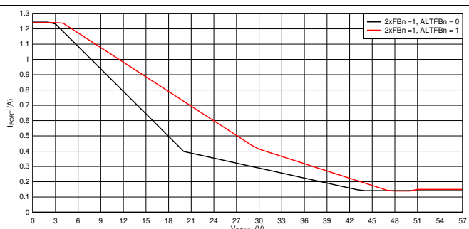
Figure 117. 2x Mode (2xFBn = 1) Foldback Curves, I PORT vs V DRAIN
