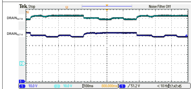
Figure 133. 4-Pair Low Resistance ( 11\text{k}\Omega ) Detection Signature
