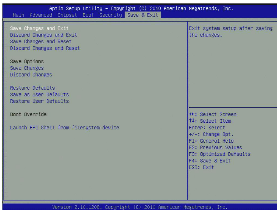
Figure 3.28 Save & Exit
