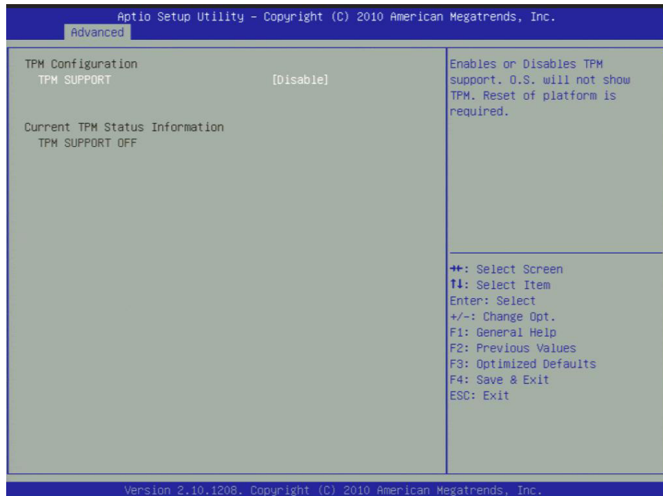
Figure 3.5 TPM Configuration
