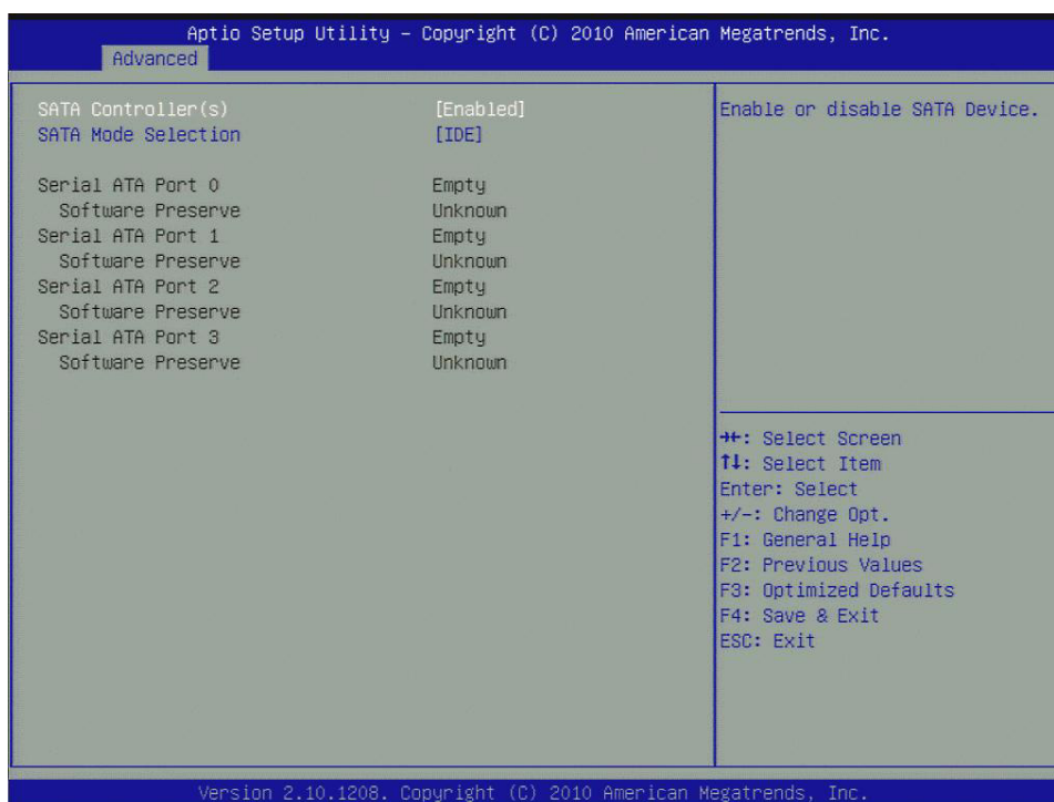
Figure 3.7 SATA Configuration
