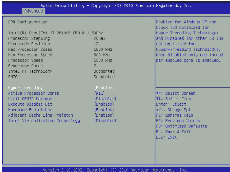
Figure 3.6 CPU Configuration
