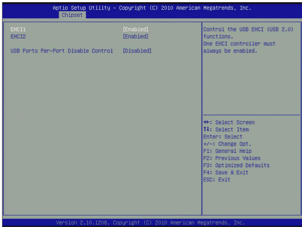
Figure 3.24 USB Configuration
