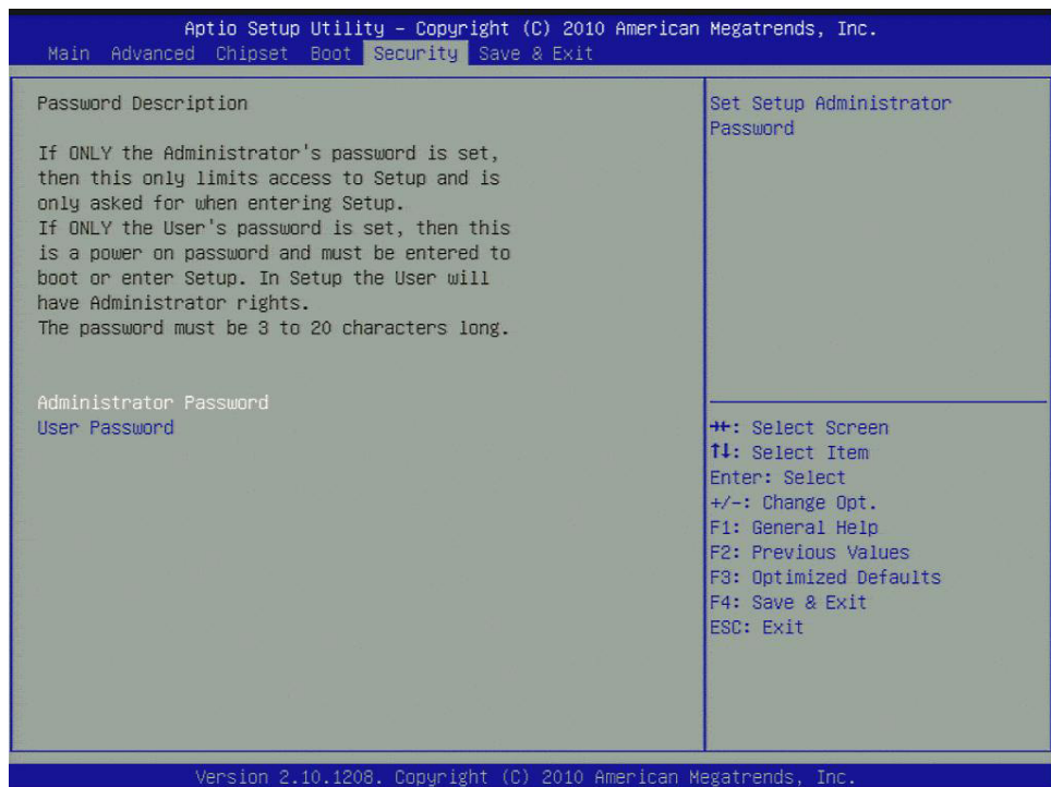
Figure 3.27 Password Configuration
