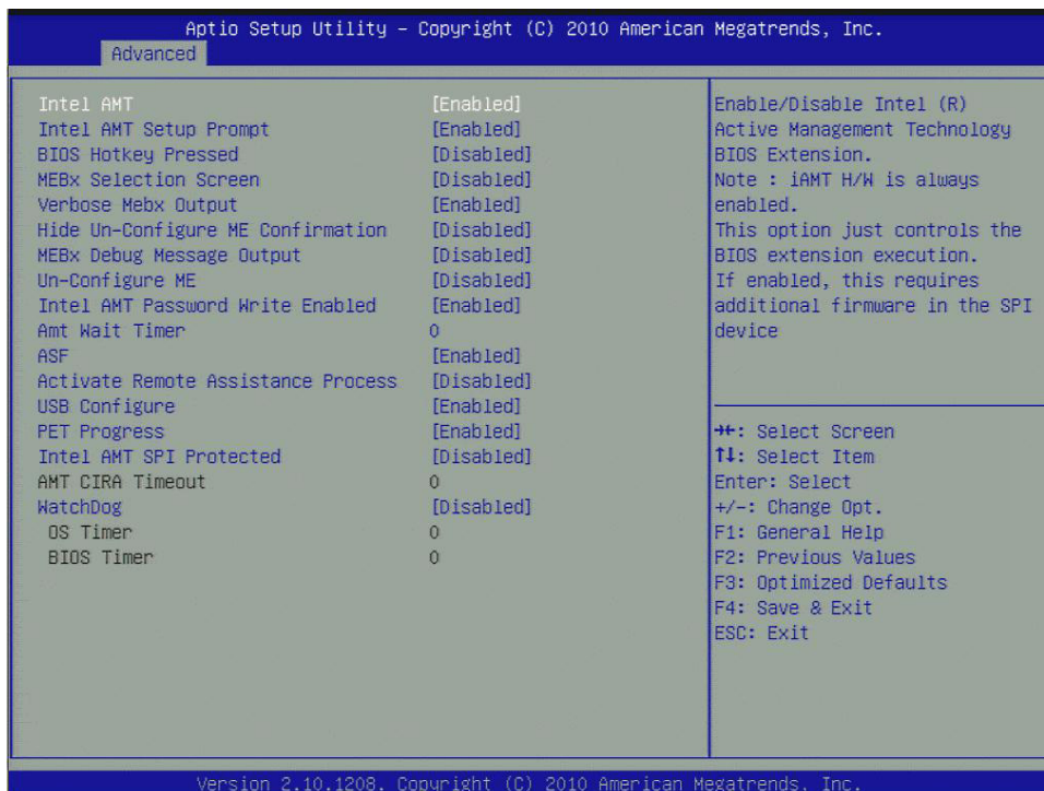
Figure 3.10 AMT Configuration
