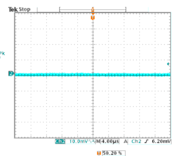
High Line, Full Load Ripple current= (2.8/10) \times 20=7.6\text{mA}
