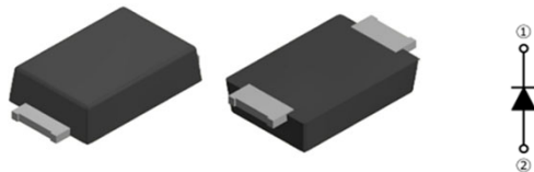
SOD-128
