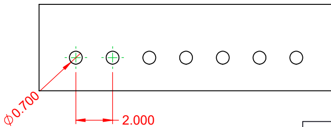
SUGGESTED PCB LAYOUT
