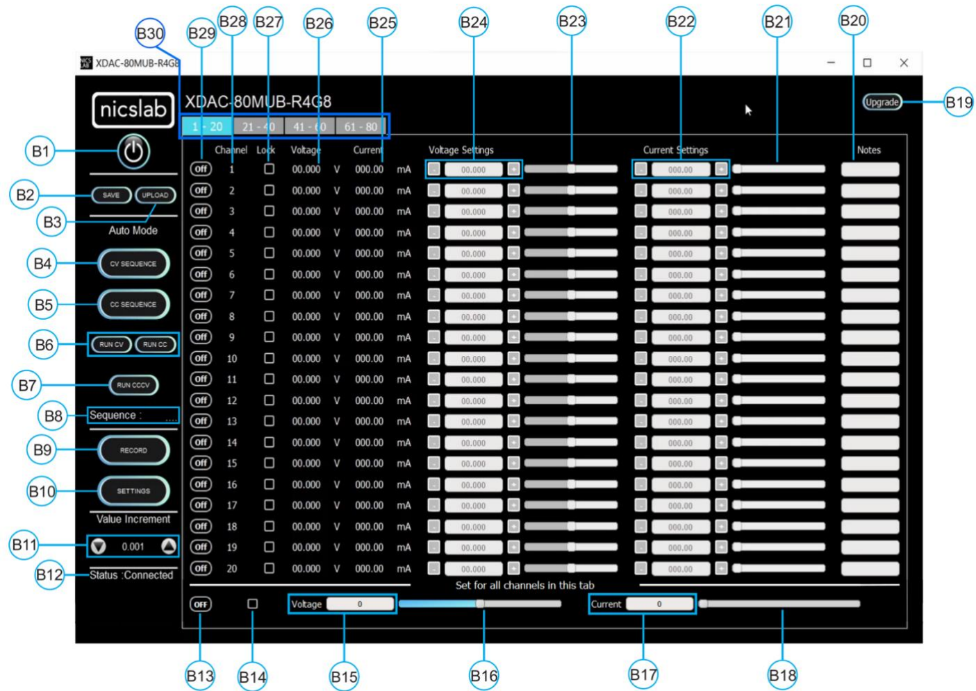
Figure 4. GUI
