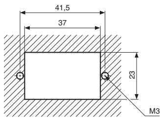
99 766 9 : Panel cut-out
