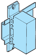
Mounting on symmetrical DIN rail EN 50022
