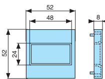
Accessory 2108 - 2108H 26 546 830
