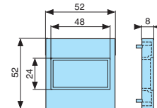
Accessory 26 546 830
