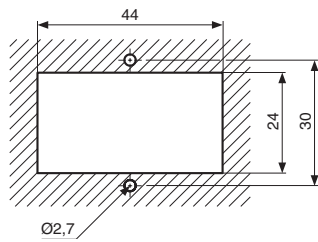
99 766 7 : Panel cut-out
