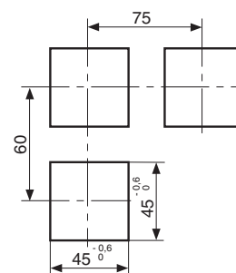
Panel cut-out
