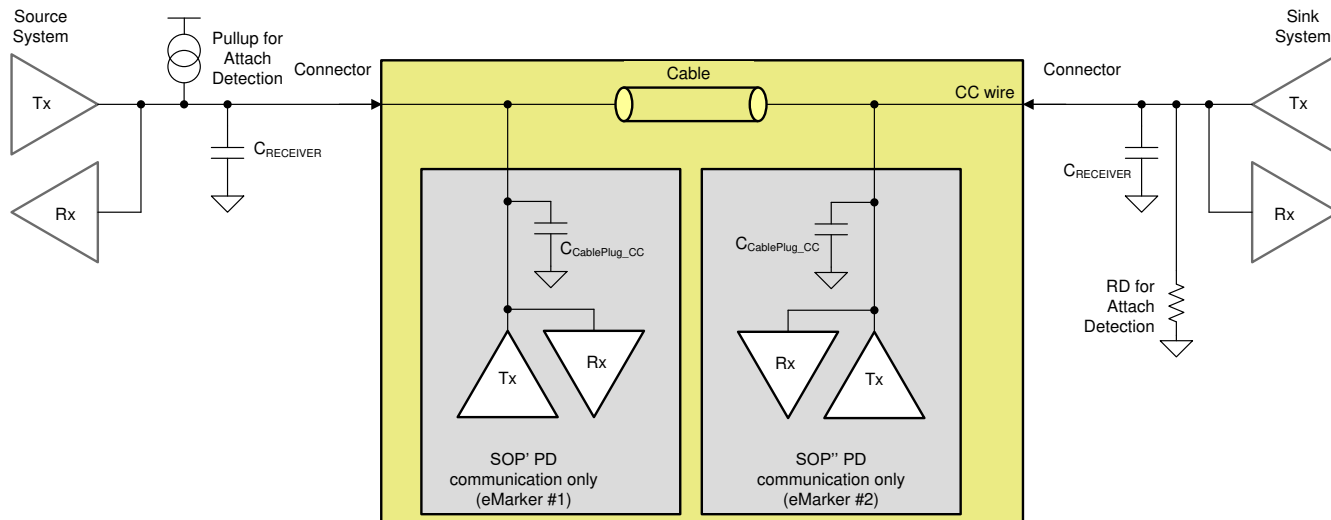
Figure 9-24. Example USB-PD Multi-Drop Configuration
