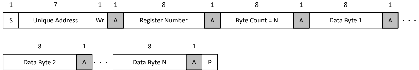
Figure 9-37. I 2 C Unique Address Write Register Protocol
