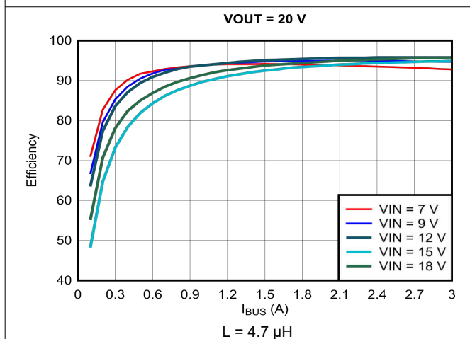
Figure 10-10. Efficiency vs Output Current ( I_{OUT} ), V_{OUT} = 20\text{ V}
