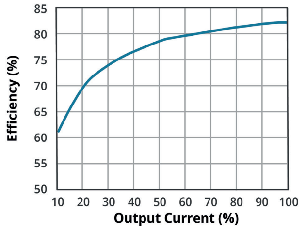
EFFICIENCY VS OUTPUT LOAD AE10-EW-S24-T
