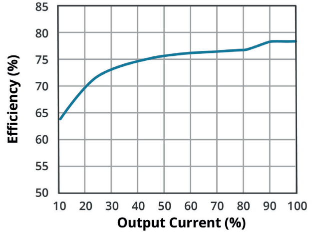
EFFICIENCY VS OUTPUT LOAD AE10-EW-S9-T
