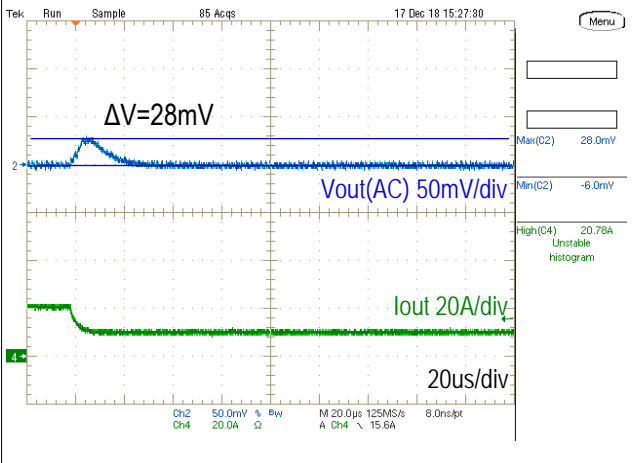
Step Load Transient Response (Vin=12.0V, Vout=1.0V, Cload=660uF, Iout=20 to 10A, 1.0A/us) Trace 2=Vout(AC), 50mV/div, Trace 4=Iout, 20A/div, 20us/div
