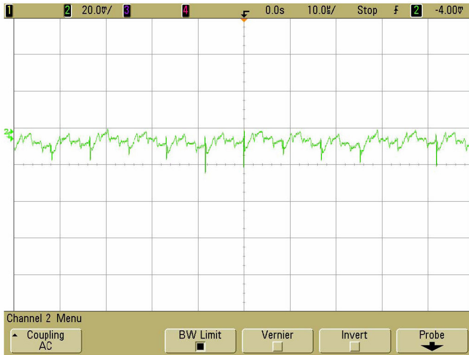
Figure 3. Output Ripple at 4.2V in and 3.0A out (20MHz) - 10uS and 20mV / div
