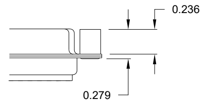
03 ..... 0.236" (MATING SIDE)
