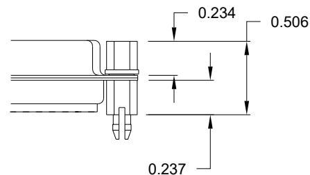
91 ..... 0.237" (SOLDER SIDE)
