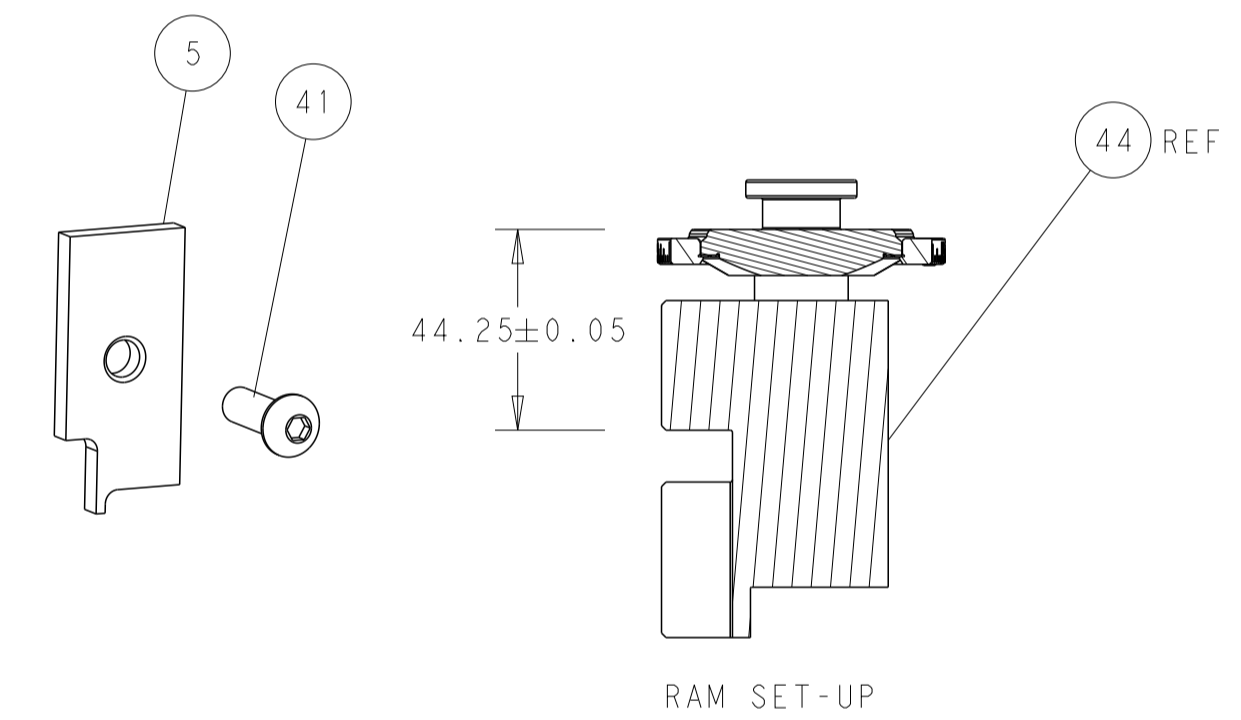
RAM SET-UP
